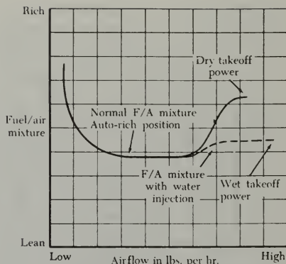
FIGURE 10-36. Fuel/air curve for a water-injection engine.
